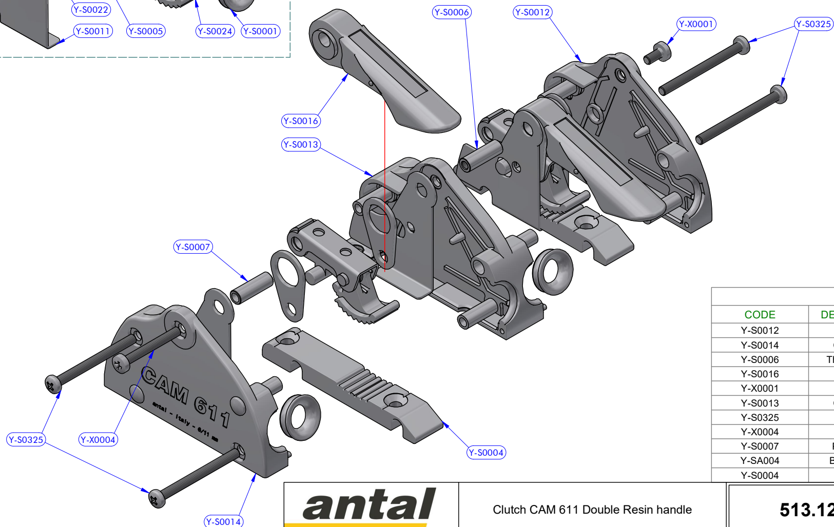
PART LIST
