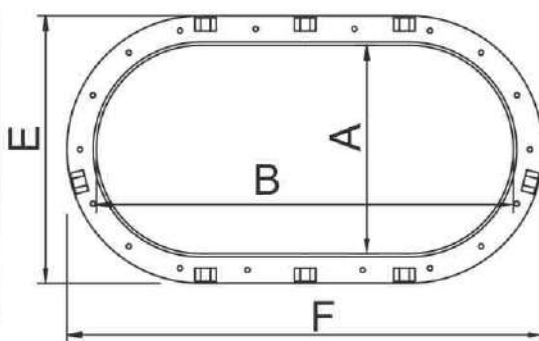
LSO-H · CLSO-H OPENING PORTHOLE
