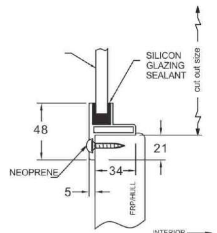
FIXED BOAT WINDOW m/m
