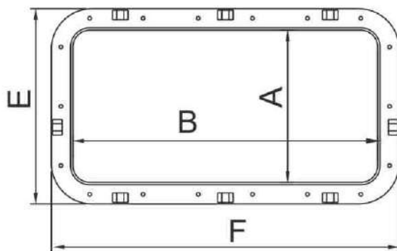
LS-H · CLS-H OPENING PORTHOLE
