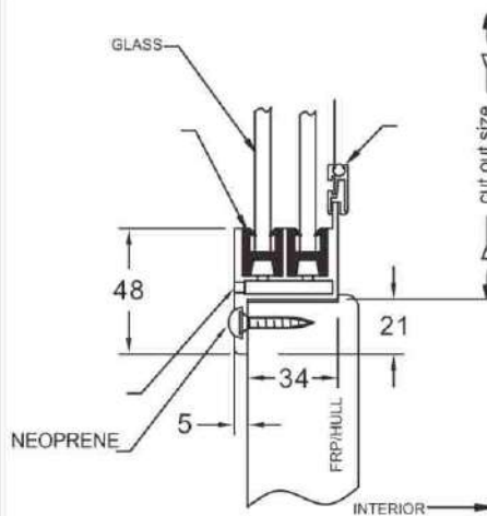
SLIDING BOAT WINDOW m/m
