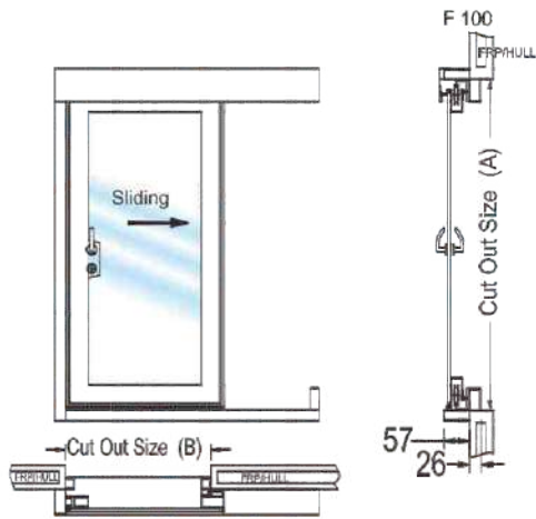
MODEL: F100 Single Sliding
