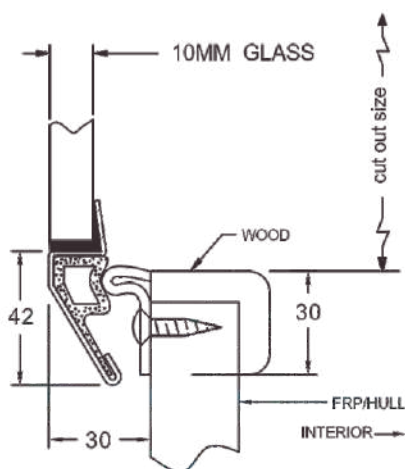
HINGED BOAT WINDOW m/m
